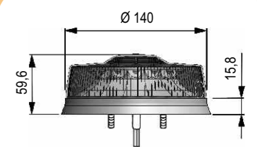
LP400 SOLARIS Dimensions in mm.
